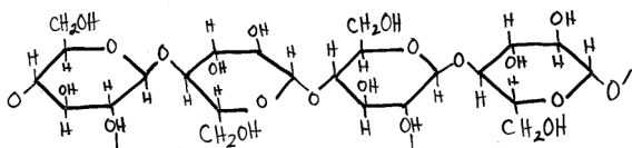
Cellulose Molecular Structure
